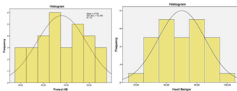
Gambar 2. Kurva data pretest-posttest hasil belajar berdistribusi normal
